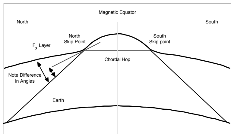
Figure 3. A diagram of a transequatorial chordal hop off the tilted north and south skip points. These points each lie between about 0^\circ and 20^\circ north and south of the Earth's magnetic equator and clearly cause nighttime TEP in the tropics.
