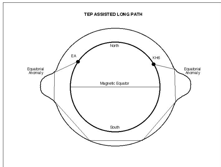
Figure 11. TEP can provide the launching points for shallow attack angle, grazing hops that cover long distances, with higher than normal MUF's and low absorption. At such times, long-path can be a superior mode of propagation.
