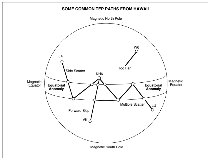
Figure 4. In geomagnetic coordinates, Hawaii is nearly due north of Australia and these TEP paths transverse north-south paths often behave like conventional skip. Signals are usually clean and stable. East-west signals from Japan and South America can have heavy scatter modulation, at times resembling aurora, and display Doppler effects as well.
