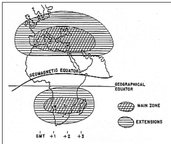
Figure 1. Path footprints for the southern Africa to Mediterranean TEP path, as seen by ZE2JV and 5B4WR in 1958 3 . (Copyright ARRL, reprinted by permission.)
