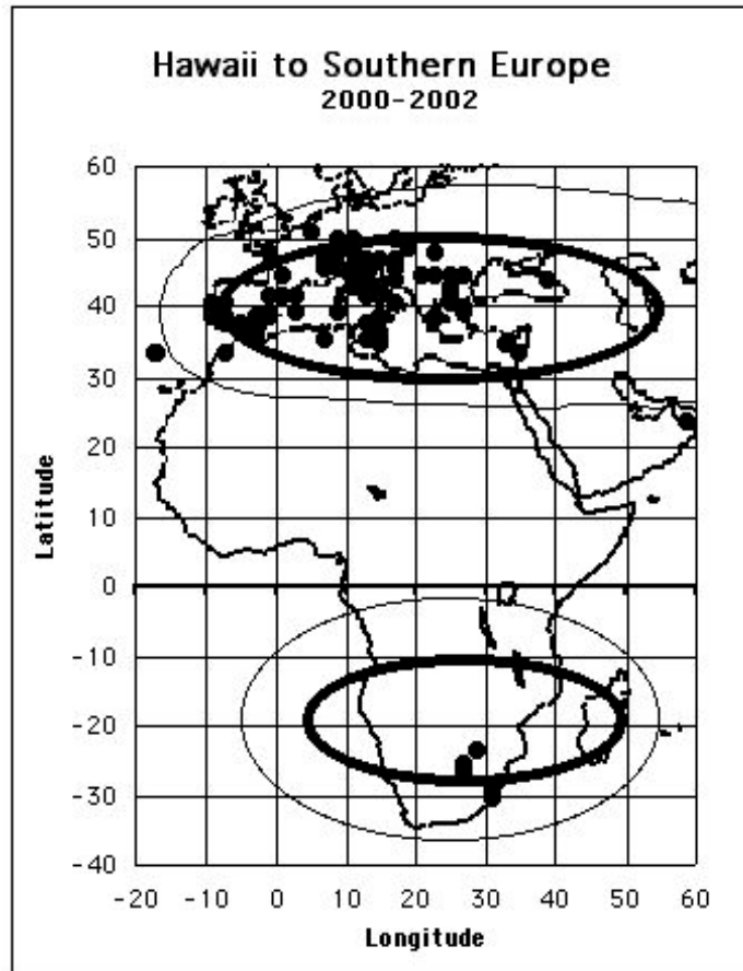
Figure 9. The footprints of the Hawaii TPL to the Mediterranean, and the non-long-path South Africa contacts. Dots show the Hawaii contacts. The ovals are the Figure 1 TEP footprints for the south African-Mediterranean path. These strongly suggest that both Hawaii propagation forms are related to some kind of TEP insertion or launching effect.
