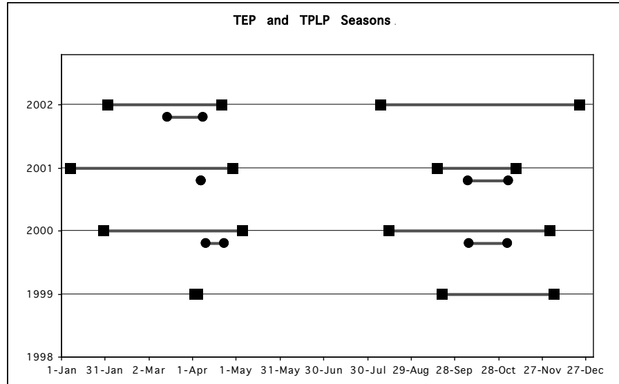
Figure 6. A diagram showing the seasonal occurrence of both TEP and TPL as found in the KH6/K6MIO log. Bars with square ends indicate the range of dates over which TEP was in evidence from time to time. Bars with round ends indicate the range of dates during which TPL was sometimes observed.
