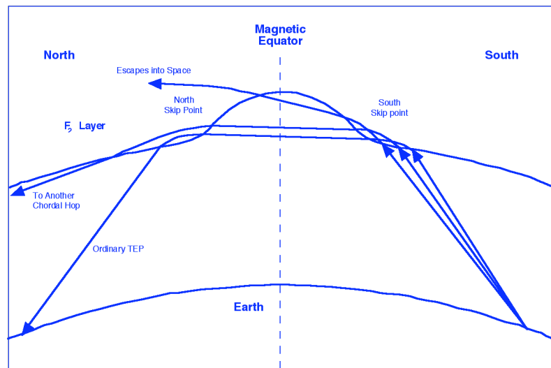
Figure 10. Refraction in the equatorial anomaly of rays transmitted at slightly different angles can lead to some parts of the signal escaping from the F 2 layer, or returning as TEP, or being injected at small angle of attack to produce further chordal hops.
