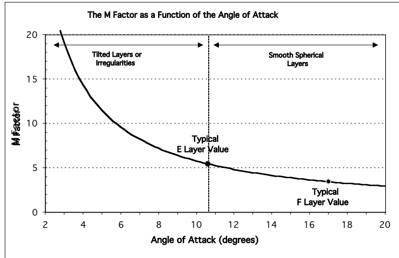
Figure 2. M ( \operatorname{cosec} \alpha ) varies with angle of attack. A smooth spherical ionosphere gives angles between 10 and 20 degrees. Tilted layers can produce lower angles, and very exciting results.
