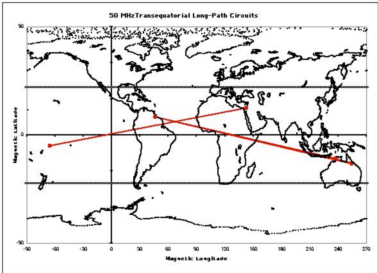
Figure 12. This map shows three examples of TEL (VK8 and VK4 overlap). The west-most station in each case is in daytime and the east-most station is in nighttime. Note that only one crossing of the magnetic equator has happened in each case. The map projection distorts the actual Great Circle routes and headings.
